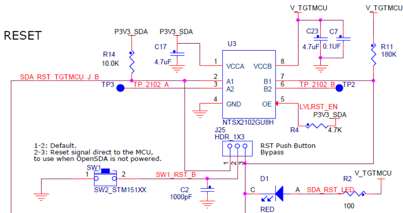
Figure 10. Reset circuit
