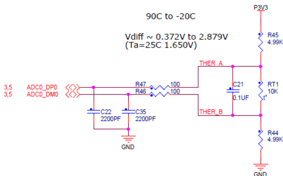
Figure 8. Thermistor
