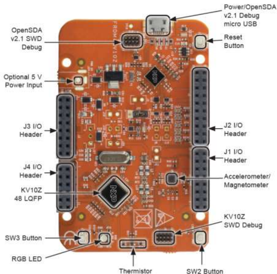
Figure 2. FRDM-KV10Z callout
