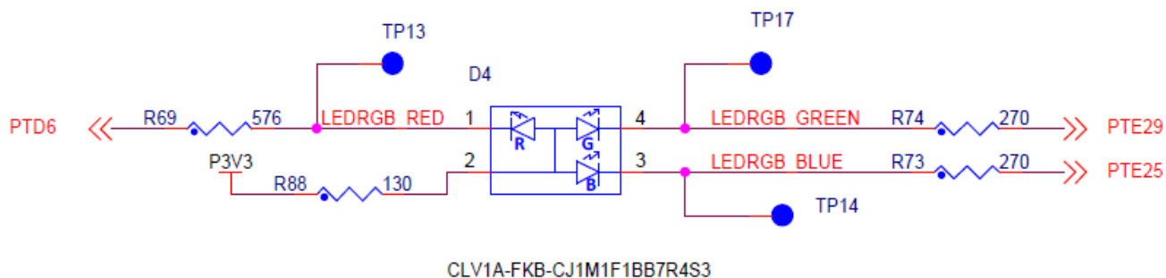
Figure 9. RGB LED
